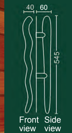
3075AB 500mm back to back set only
